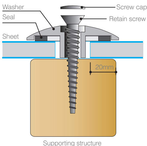
Supporting structure
